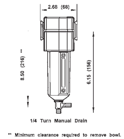
** Minimum clearance required to remove bowl.
