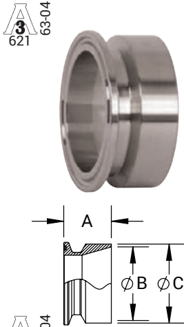
Tube O.D. Clamp x Schedule 5S Weld Adapters - B19MPV
