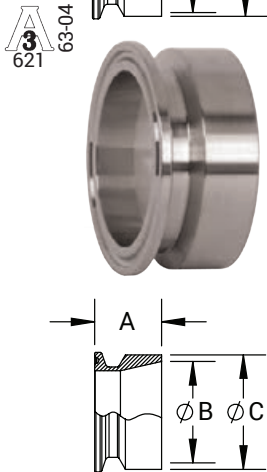
Tube O.D. Clamp x Schedule 10S Weld Adapters - B19MPX
